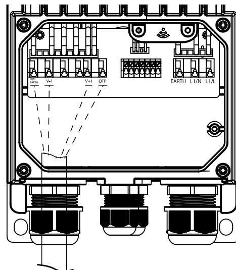
Floodlight Driver Box
