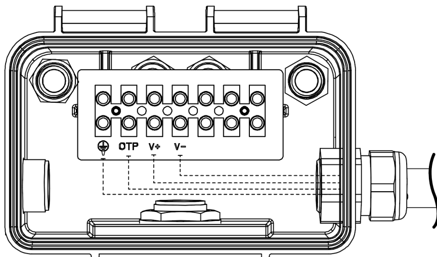
Floodlight Junction Box
